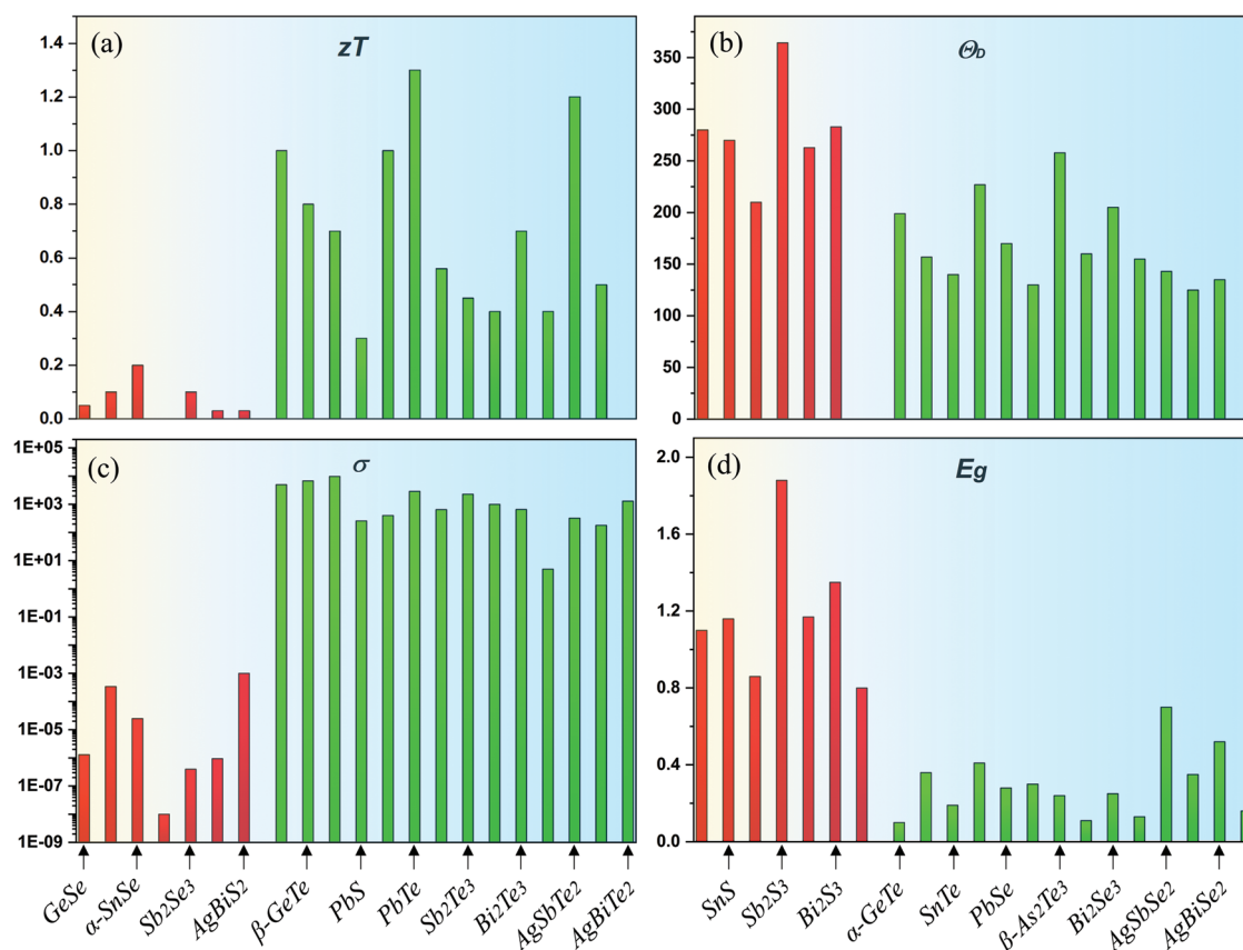
Figure 1. Characteristic properties of pristine chalcogenide compounds listed in Table 1. a) Maximum zT values; b) Debye temperature in Kelvin; c) Electrical conductivity at room temperature in \text{S cm}^{-1} ; d) Bandgap in eV. These materials can be divided into two groups regarding their performance as thermoelectrics: materials with zT values larger than 0.25 are displayed in green, while those with zT below 0.25 are depicted in red. The subgroup which possesses high figure of merits also shows a distinct property portfolio, including a low Debye temperature, high electrical conductivity, and small bandgap.
