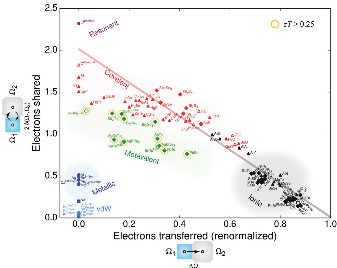
Figure 2. A 2D map of electronic interactions and bonding in materials. The amount of relative electrons transferred (x-axis) and shared between neighboring basins (y-axis) is computed using quantum-topological methods. Please note that the number of electrons transferred has been divided by the formal oxidation state to obtain the relative charge transfer. A relative electron transfer of 1 thus corresponds to the transfer of one electron in NaCl but two electrons in MgO. The different colors denote that the corresponding materials have different properties (structure, electrical conductivity, optical dielectric constant, anharmonicity, and bond polarizability) which are indicative for different bonding mechanisms, i.e., ionic (black), covalent (red), metallic (blue), van der Waals (light blue), and resonant bonding as in graphite or benzene (purple). Materials with an unconventional property portfolio (high values of \epsilon_{\infty} , an intermediate electrical conductivity, large anharmonicities, pronounced electron–phonon coupling, and an effective coordination number incompatible with ordinary covalent bonding) are denoted in green. Their properties have been attributed to an unconventional bonding mechanism which has been coined metavalent bonding. Interestingly, all octahedrally coordinated chalcogenides with a zT above 0.25 for their intrinsic phases are located in the green region. This implies that there could be a correlation between their thermoelectric performance and the bonding mechanism utilized. The map can be employed to identify novel thermoelectrics.
